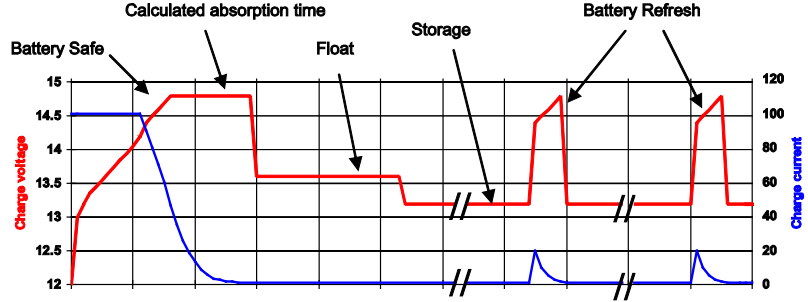
Figure 3: Four-step adaptive charge curve
